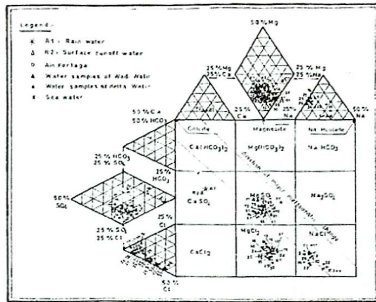
Fig. (3). Durov's diagram of the groundwater samples of alluvium aquifer in wadi Watir and its delta.
