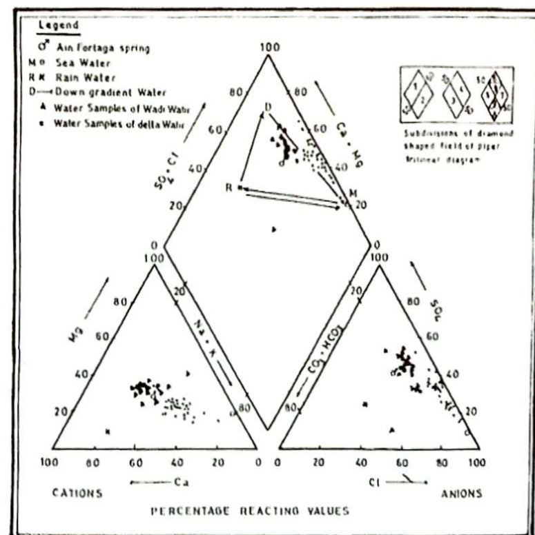
Fig. (2). Piper's diagram for the groundwater samples of alluvium aquifer in wadi Watir and its delta.
