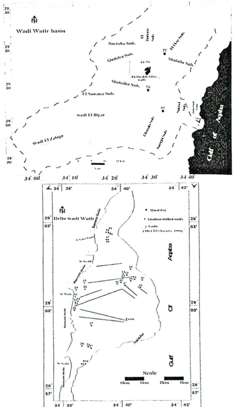
Fig. (1). Well location map of the groundwater samples of alluvium aquifer in wadi Watir and its delta.
