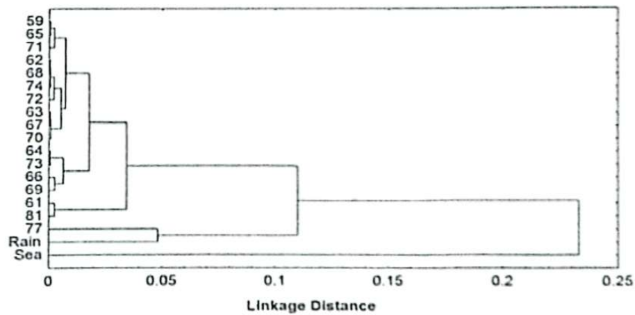
Tree Diagram for 19 Cases, Complete linkage (1-Pearson r)
