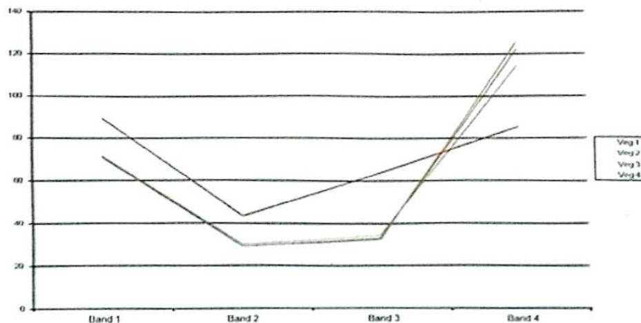
Fig. (5). Mean plot of signatures.
