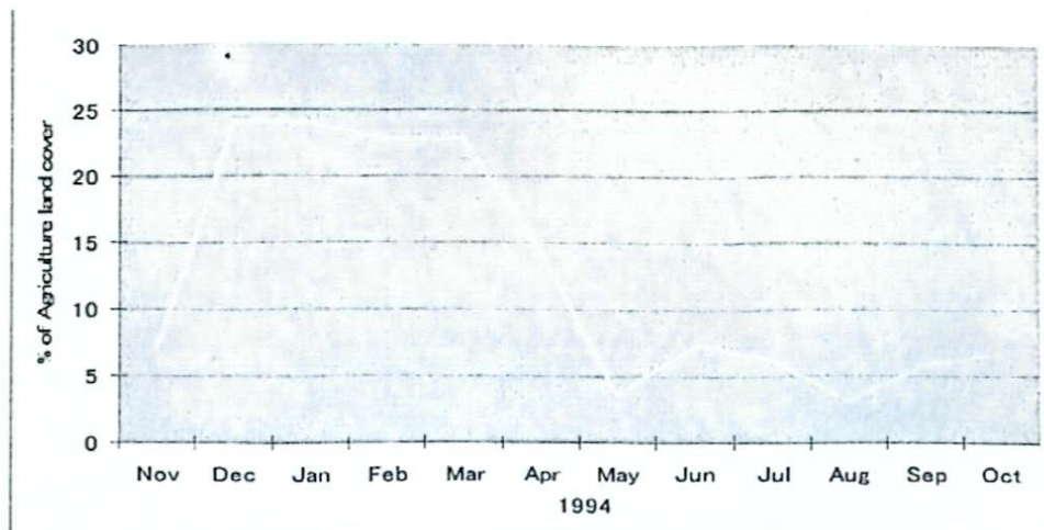
Fig. (8). Agricultural cover transition of Al Qassim area along Wadi Ar Rumah from Landsat TM data analysis.
