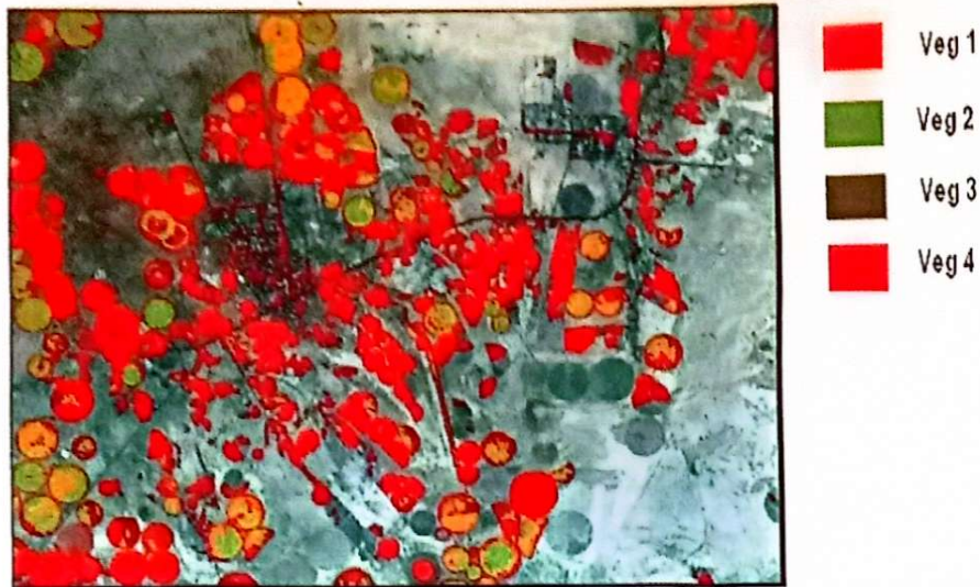
Fig. (6). The classified image obtained using Maximum Likelihood classifier of February, 1994. Veg 1 denotes to alpha alpha, Veg 2 barley, Veg 3 palm tree, Veg 4 Wheat.
